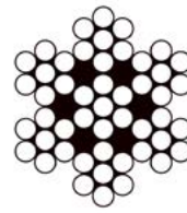
7X7
